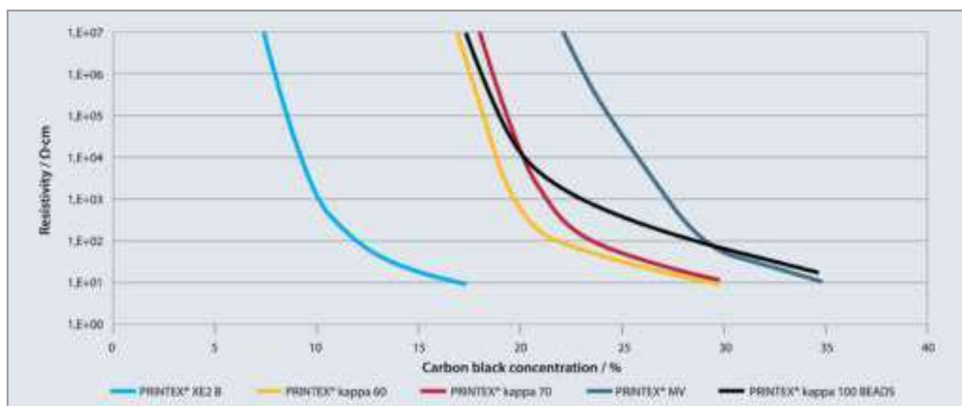
Percolation curves will differ depending on the polymer and process used. Below example of the performance of different conductive carbon blacks in PE-LD injection molded plaques
