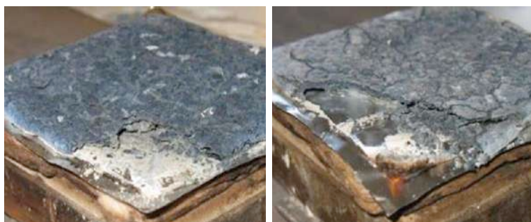
Above: Images showing the improved char formation resulting from the addition of 3% of Evonik’s Tegomer FR100 additive in a cable compound sample (right)
