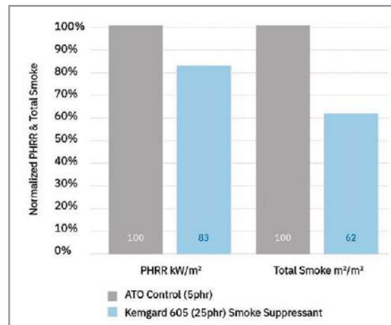
Figure 2: Replacing equal parts of CaCO 3 +ATO + zinc borate in a PVC cable compound with Kemgard 605 results in reduced smoke generation and improved fire performance
