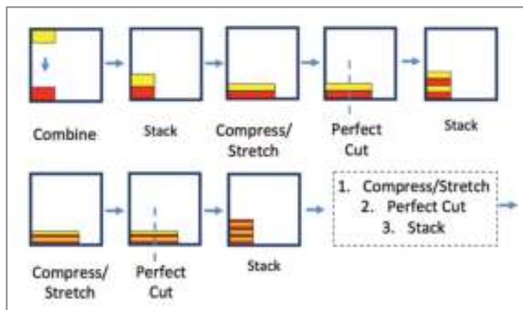
Figure 1: A schematic representation showing the basic principle of the Baker's Transformation in melt mixing Source: Randcastle Extrusion Systems
