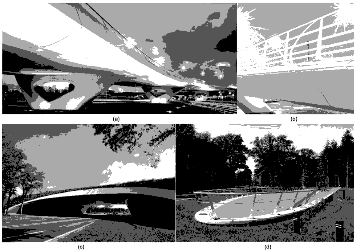
Fig. 9. Some projects in the Netherlands with FRP edge elements. (a) The fly-over Waarderpolder in Haarlem; (b) edge elements on the Juliana Bridge in Zaanstad; (c, d) the wildlife crossing and tunnel in Rijssen-Wierden (Royal HaskoningDHV, 2007, 2013, 2013).
