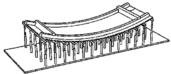
Fig. 6. A flexible mold system for cambered decks with variable width and length.
