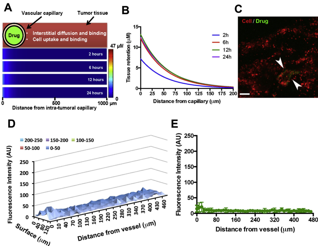
Fig. 2. Computational modeling of drug delivery to pancreatic tumors. (A) Layout of the computational domain consisting of a single vascular capillary (in pink) from which intravenous delivered drug (green) is transported into the surrounding tumor tissue (red) and distributes via interstitial diffusion/binding and cell uptake/binding. Underneath is represented the presence of drug over a time course of 24 h within the tumor mass. (B) Linear representation of tissue distribution predicts that drug will reach tumor site at a very limited concentration. (C) Confocal imaging of a tumor tissue section after 14 days treatment consisting of weekly injection of paclitaxel-Cremophore formulation. Image taken two hours after intravenous injection highlights presence of the fluorescent paclitaxel only at the lumen/tissue interface (Bar = 100 \mu\text{m} ). (D) Analysis of the fluorescence intensity at the surface. (E) Fluorescence intensity are in accordance with computational prediction of very limited drug penetration (data shown are displayed as mean \pm standard deviation). (For interpretation of the references to colour in this figure legend, the reader is referred to the web version of this article.)
