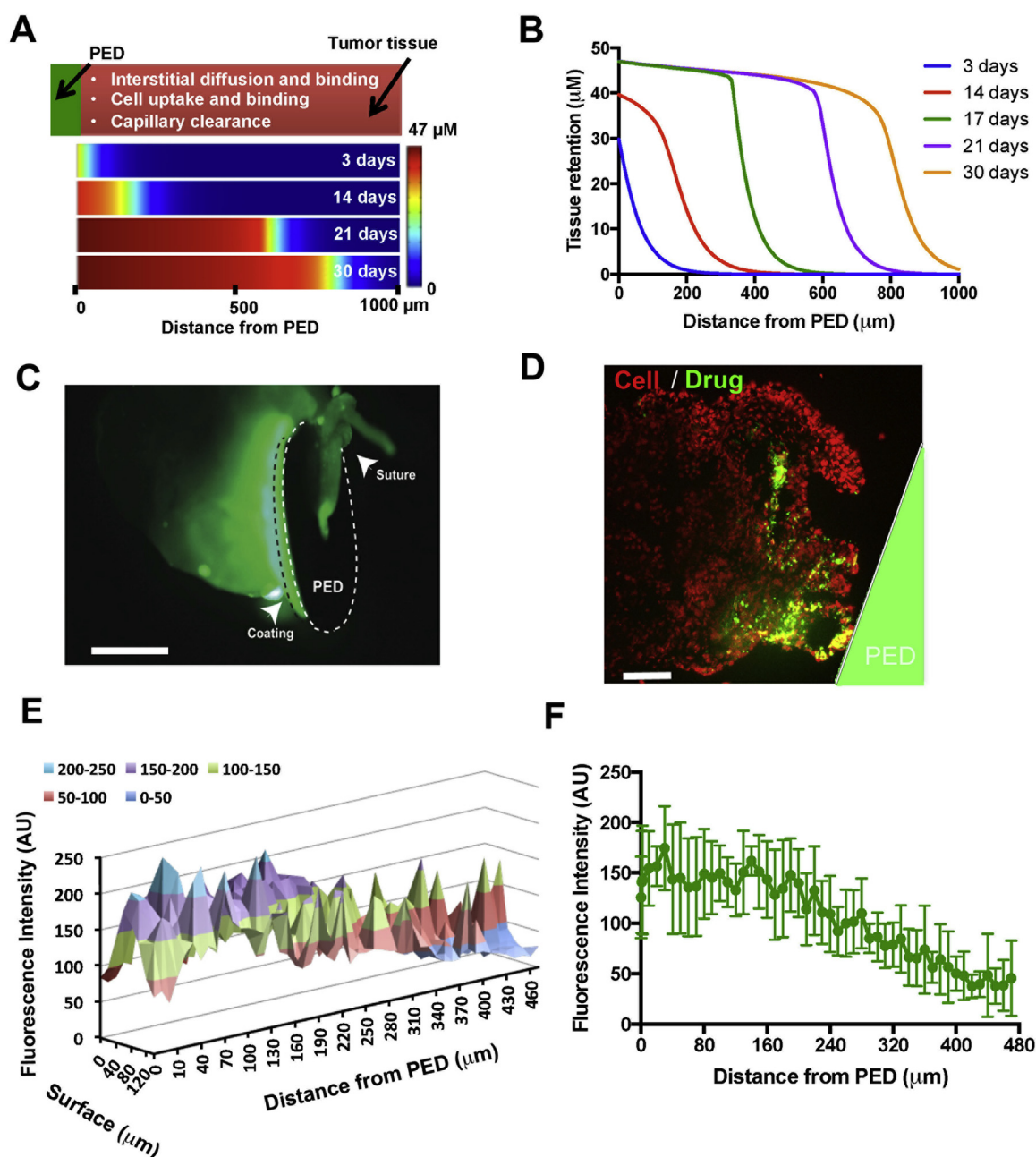
Fig. 4. Localized therapeutic strategy implementing PED greatly enhances intratumoral deliverability of chemotherapeutic agents. (A) Schematic of the computational domain consisting of a confined tumor tissue (red), the device as source of drug (green) taking into consideration interstitial diffusion/binding, cell uptake/binding and capillary clearance. Underneath is represented drug distribution over a course of 30 days within the tumor mass. (B) Linear representation of intratumoral drug distribution predicts elevated paclitaxel tissue retention as a function of release kinetics and extended over 1 mm after 30 days of treatment. (C) Representative fluorescent image under a dissecting microscope of tumor mass harvested 14 days post-treatment points out a macroscopic drug presence (Bar = 3 \mu\text{m} ). (D) Confocal analysis of tumor tissue sections highlight the extensive penetration of the drug at increased distance from the tumor/PED interface (Bar = 100 \mu\text{m} ). Image represents a time point of 14 days post-implant of the PED. (E) Surface analysis and (F) Fluorescent intensity from tissue was in accordance with computational predictions of drug penetration after 14 days of treatment (data in are displayed as mean \pm standard deviation). (For interpretation of the references to colour in this figure legend, the reader is referred to the web version of this article.)
