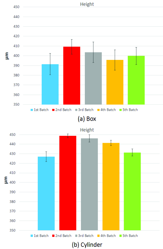
Fig. 4 Height measurement for (a) box and (b) cylinder
